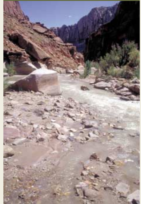
Figure 37. Coarse-textured soil and channel bed material are more susceptible to lateral migration.
